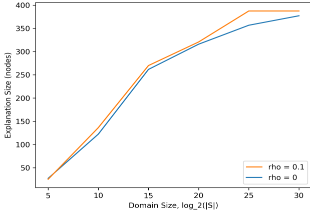
Figure 6: Comparison of explanation versus state-space size.
